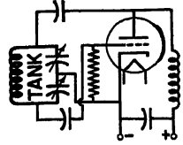
Colpitts oscillator circuit.
